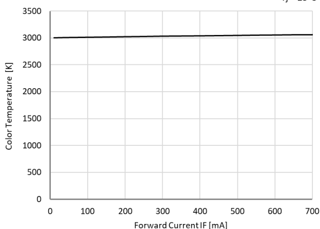
Forward Current vs. Color Temperature
